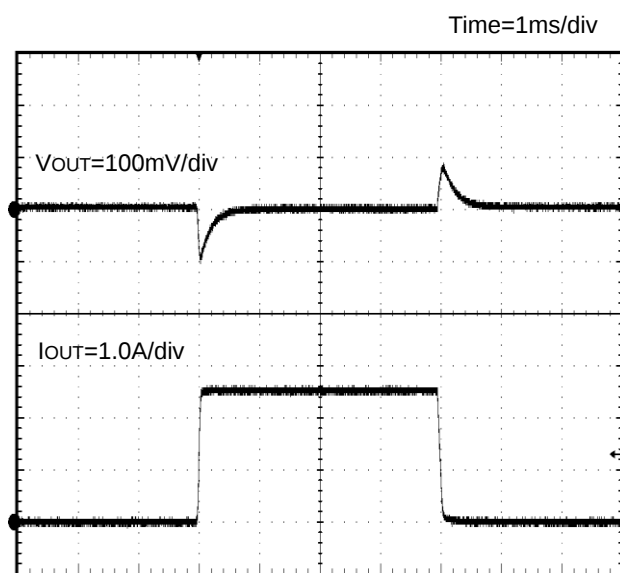
Figure 39. Load Transient Response I_{OUT}=0A - 2.5A ( V_{IN}=12V , V_{OUT}=3.3V , C_{OUT}=\text{Ceramic}22\mu F \times 2 )
