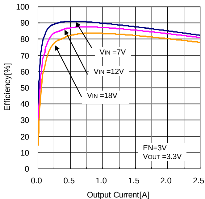
Figure 18. Efficiency vs Output Current ( V_{OUT} = 3.3V , L = 4.7\mu H )
