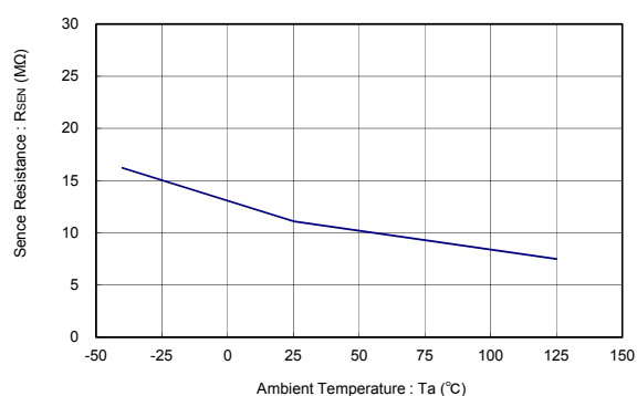
XC6133 ( V_{DF(T)}=1.0V )
