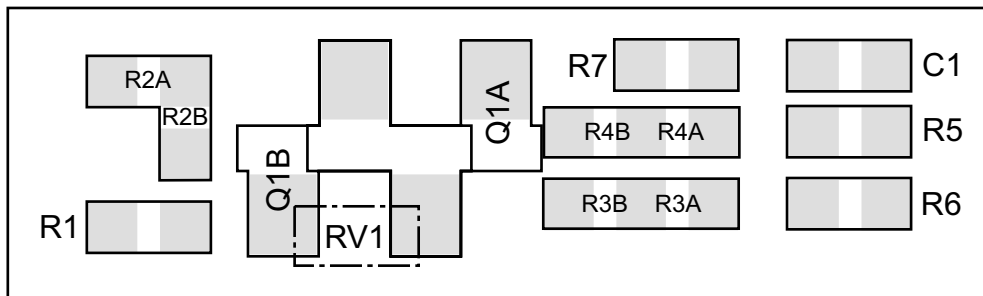
Figure 3.2 One-Transistor Cell
