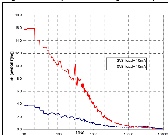
Figure 14. Output noise voltage vs. frequency
