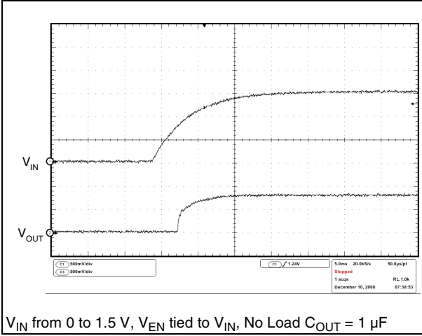
Figure 16. Startup transient
