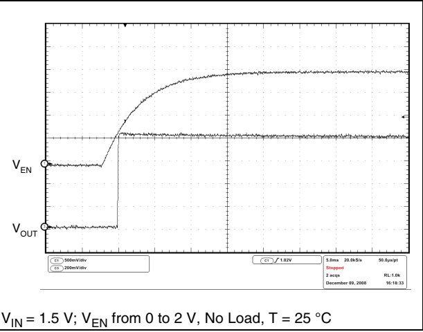
Figure 17. Enable transient
