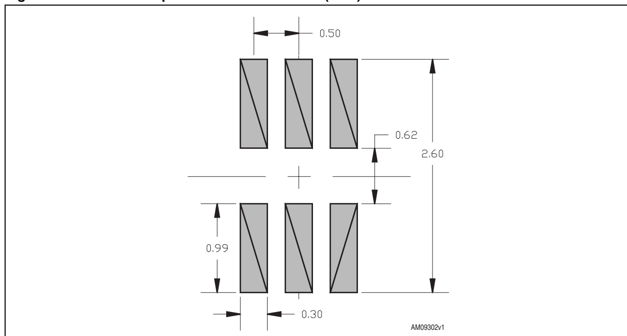
Figure 19. SOT666 footprint recommended data (mm.)
