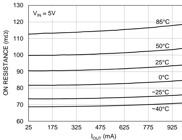
Figure 6 On-Resistance vs. I_{OUT} and Temperature
