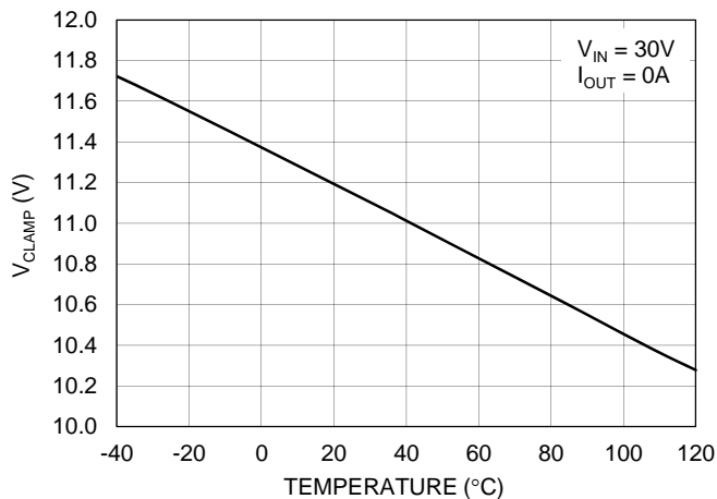
Figure 4 Output Clamp Voltage vs. Temperature
