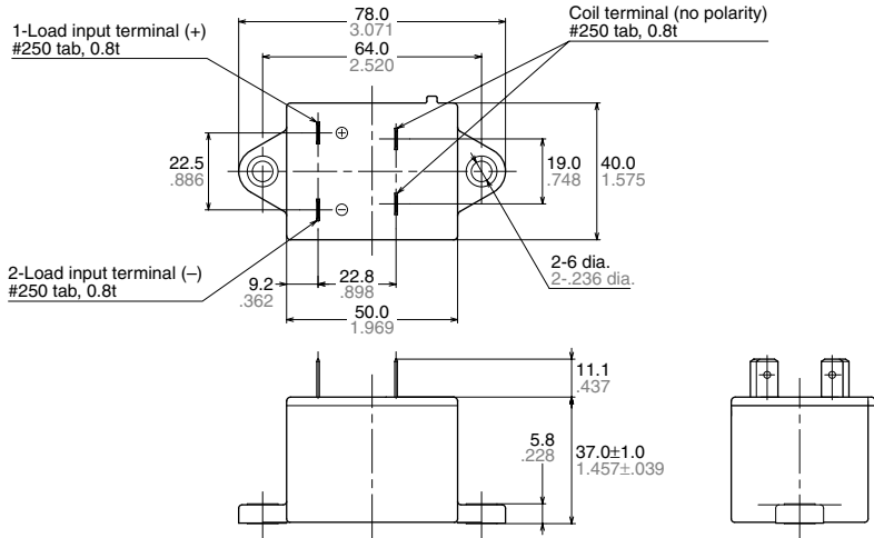
External dimensions
