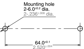
Panel cut-off
