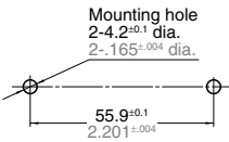
Panel cut-off
