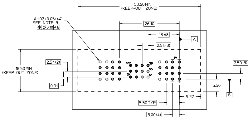
RECOMMENDED PCB LAYOUT AND KEEP-OUT ZONE
