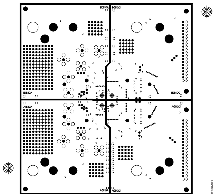
Figure 27. GND2
