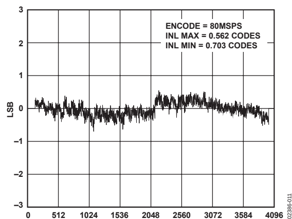
Figure 12. Integral Nonlinearity
