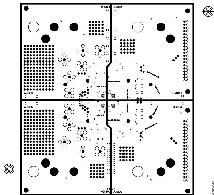
Figure 26. GND1
