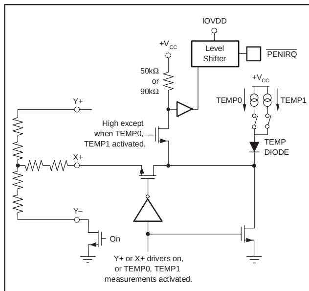
Figure 10. PENIRO Functional Block Diagram
