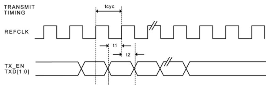
Figure 19. RMII Timing – Data Received from RMII
