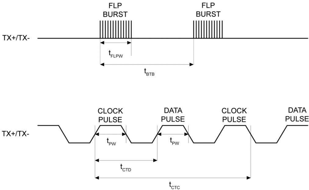
Figure 23. Auto-Negotiation Timing
