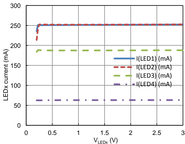
Figure 13 LEDx Current vs. V_{LEDx}
