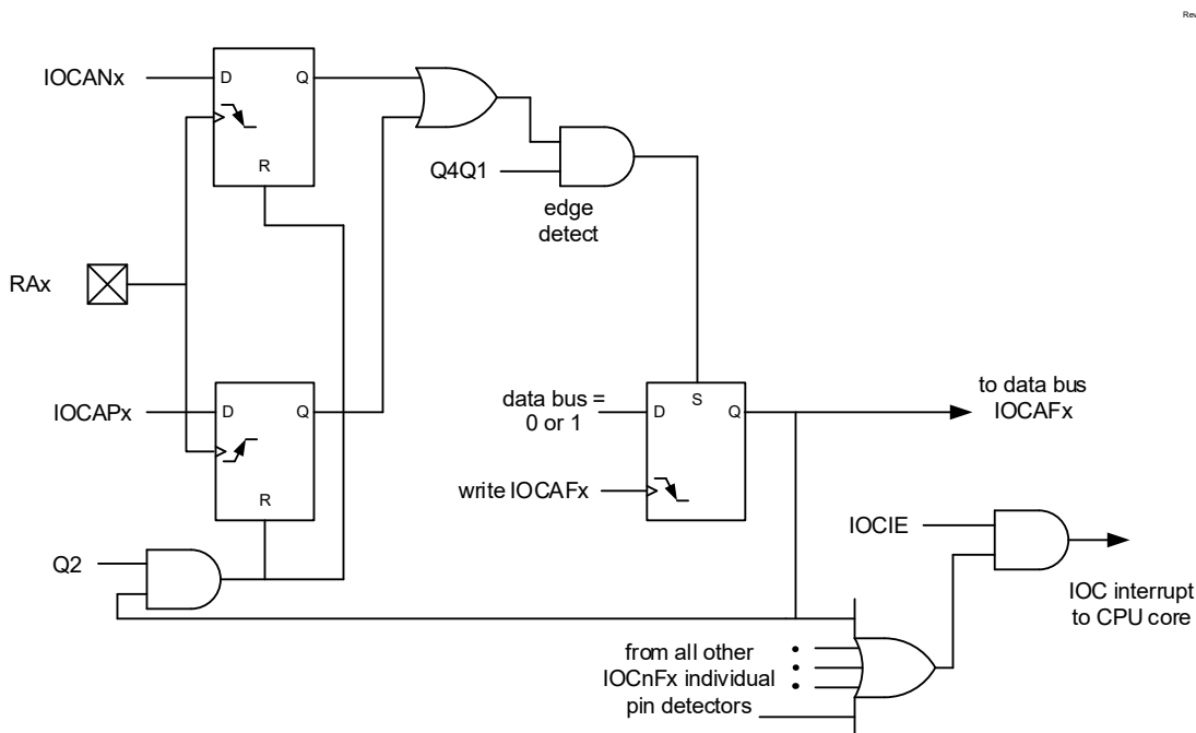
Figure 17-1. Interrupt-on-Change Block Diagram (PORTA Example)
