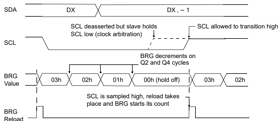
Figure 35-25. Baud Rate Generator Timing with Clock Arbitration
