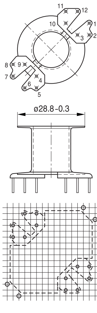
Hole arrangement View in mounting direction
