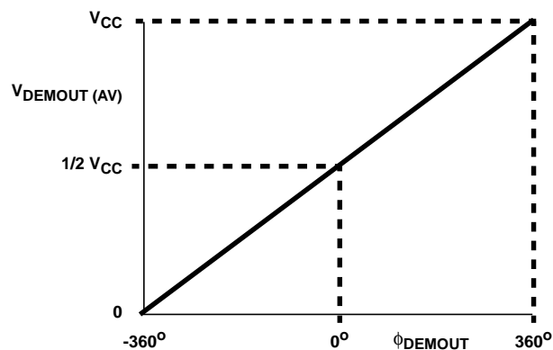
FIGURE 4. PHASE COMPARATOR 2: AVERAGE OUTPUT VOLTAGE vs INPUT PHASE DIFFERENCE: V_{\text{DEMOUT}} = V_{\text{PC2OUT}} = (V_{\text{CC}}/\pi) (\phi_{\text{SIGIN}} - \phi_{\text{COMPIN}}) \phi_{\text{DEMOUT}} = (\phi_{\text{SIGIN}} - \phi_{\text{COMPIN}})
