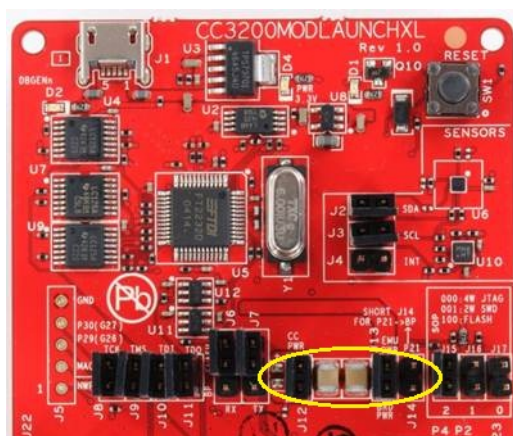
Figure 9. Powering From USB
