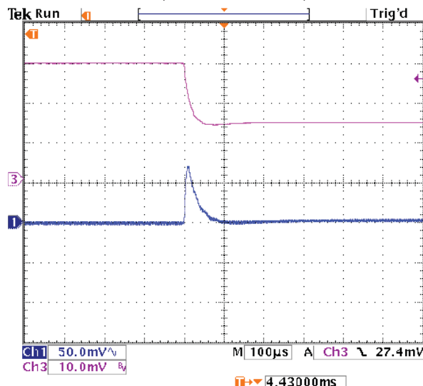
Step Load Transient Response (Vin=12V, Vout=5V, Clload=0, Iout=3A to 1.5A) Trace 1=Vout, 50 mV/div. Trace 3=Iout, 1A/div.
