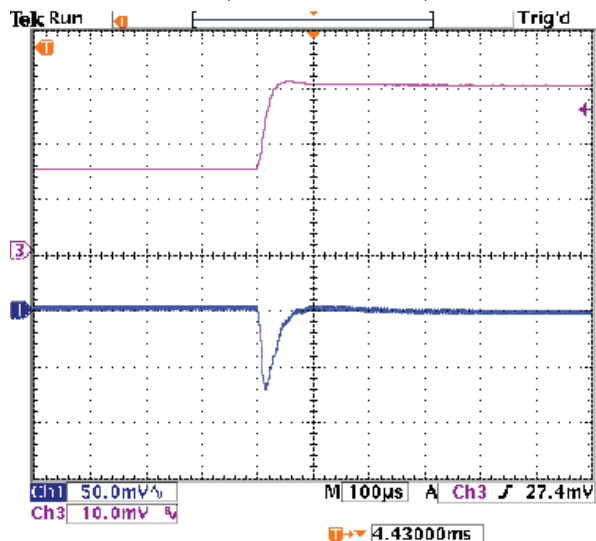
Step Load Transient Response (Vin=12V, Vout=5V, Clload=0, Iout=1.5A to 3A) Trace 1=Vout, 50 mV/div. Trace 3=Iout, 1A/div.
