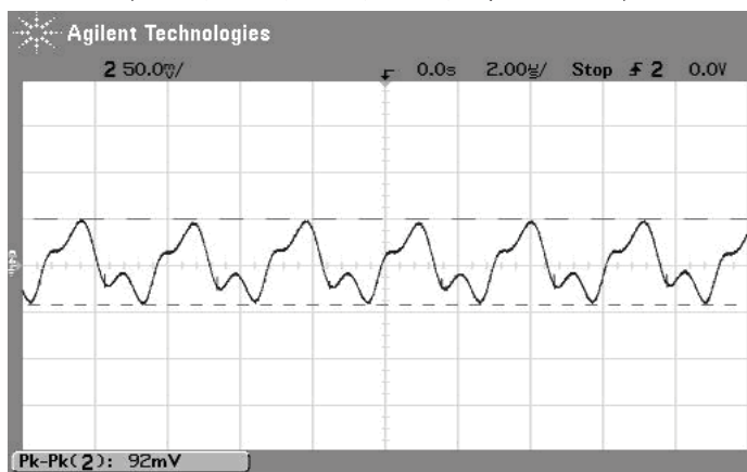
Output Ripple and Noise (Vin=12V, Vout=5V, Iout=5A, Clload=0, ScopeBW=100MHz)
