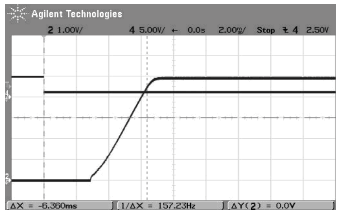
On/Off Enable Startup Delay (Vin=12V, Vout=5V, Iout=3A, Load=0) Trace 4=Enable In, Trace2=Vout
