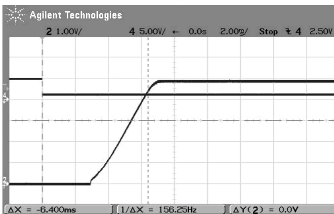
On/Off Enable Startup Delay (Vin=12V, Vout=5V, Iout=5A, Clload=0 Trace 4=Enable In, Trace2=Vout)
