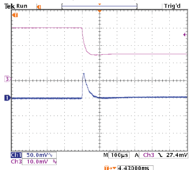
Step Load Transient Response (Vin=12V, Vout=5V, Load=0, Iout=3A to 1.5A) Trace 1=Vout, 50 mV/div. Trace 3=Iout, 1A/div.
