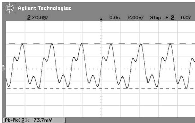
Output Ripple and Noise (Vin=12V, Vout=5V, Iout=3A, Load=0, ScopeBW=100MHz)
