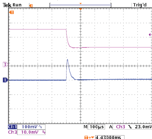
Step Load Transient Response (Vin=12V, Vout=5V, Clload=0, Iout=5A to 2.5A) Trace 1=Vout, 100 mV/div. Trace 3=Iout, 2A/div.
