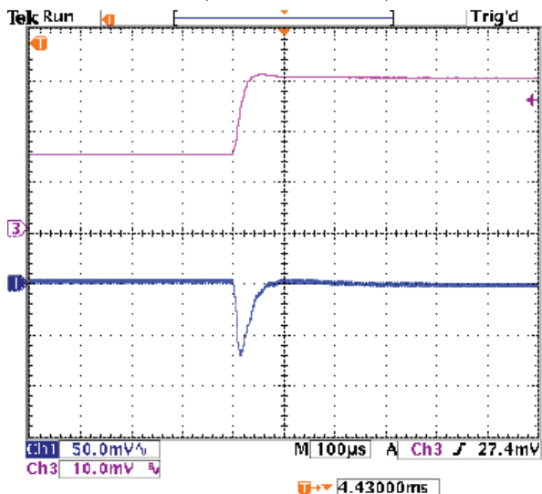
Step Load Transient Response (Vin=12V, Vout=5V, Load=0, Iout=1.5A to 3A) Trace 1=Vout, 50 mV/div. Trace 3=Iout, 1A/div.
