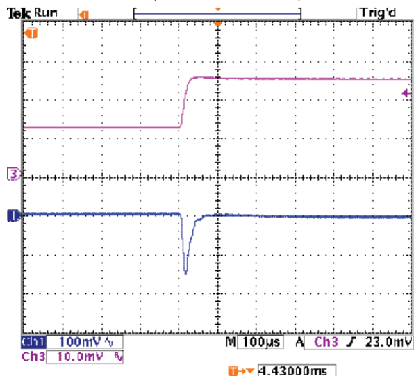
Step Load Transient Response (Vin=12V, Vout=5V, Clload=0, Iout=2.5A to 5A) Trace 1=Vout, 100 mV/div. Trace 3=Iout, 2A/div.
