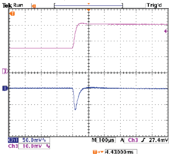
Step Load Transient Response (Vin=12V, Vout=1.2V, Clad=0, Iout=1.5A to 3A) Trace 1=Vout, 50 mV/div. Trace 3=Iout, 1A/div.
