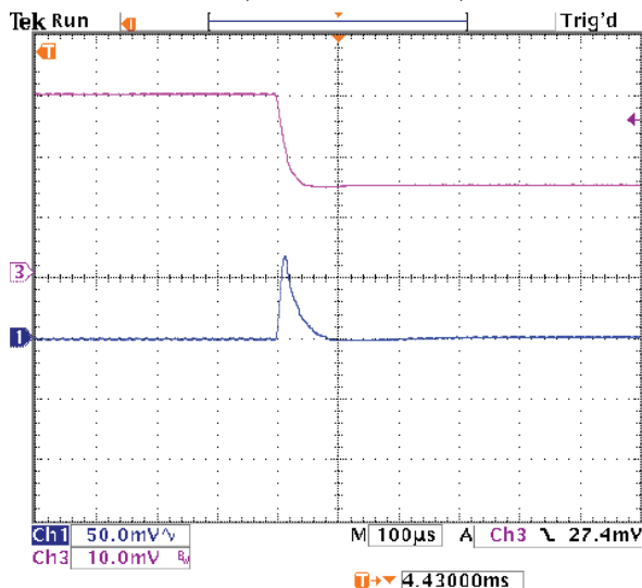
Step Load Transient Response (Vin=12V, Vout=1.2V, Clad=0, Iout=3A to 1.5A) Trace 1=Vout, 50 mV/div. Trace 3=Iout, 1A/div.
