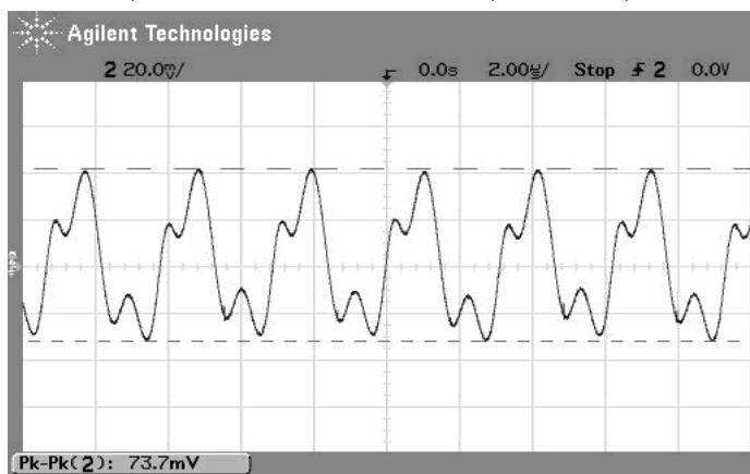
Output Ripple and Noise (Vin=12V, Vout=5V, Iout=3A, Clod=0, ScopeBW=100MHz)
