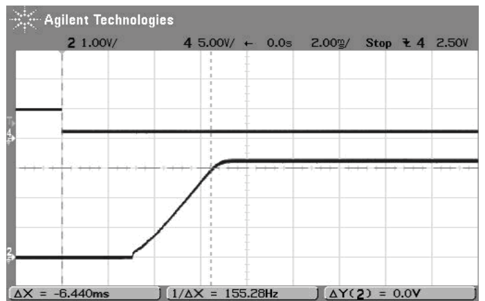
On/Off Enable Startup Delay (Vin=12V, Vout=3.3V, Iout=5A, Cload=0) Trace 4=Enable In, Trace 2=Vout
