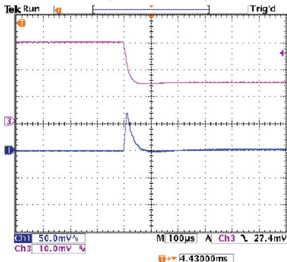
Step Load Transient Response (Vin=12V, Vout=2.5V, Cload=0, Iout=3A to 1.5A) Trace 1=Vout, 50 mV/div. Trace 3=Iout, 1A/div.
