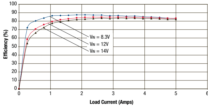
OKY-T/5-D12 Efficiency vs. Line Voltage and Load Current @ 25°C (Vout = 1.2V)
