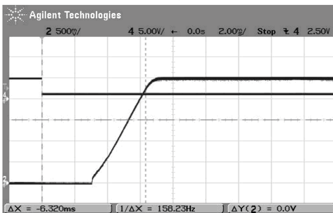
On/Off Enable Startup Delay (Vin=12V, Vout=2.5V, Iout=3A, Cload=0) Trace 4=Enable In, Trace 2=Vout
