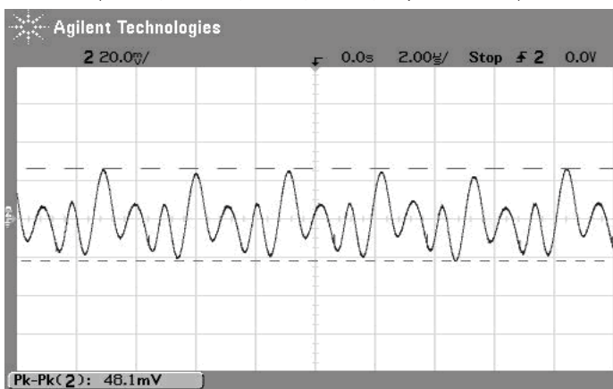
Output Ripple and Noise (Vin=12V, Vout=1.2V, Iout=3A, Clad=0, ScopeBW=100MHz)
