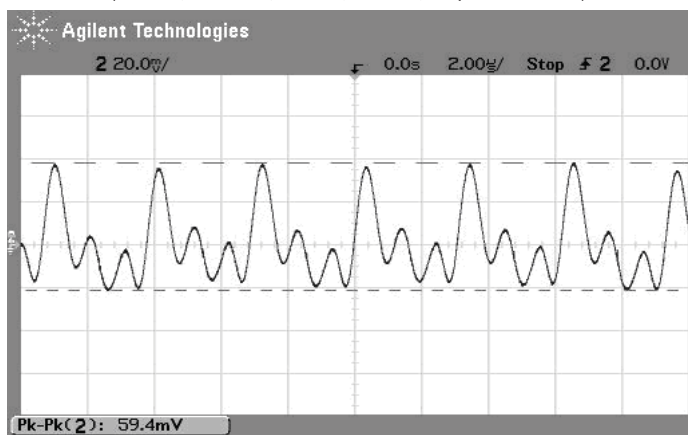
Output Ripple and Noise (Vin=12V, Vout=2.5V, Iout=3A, Cload=0, ScopeBW=100MHz)
