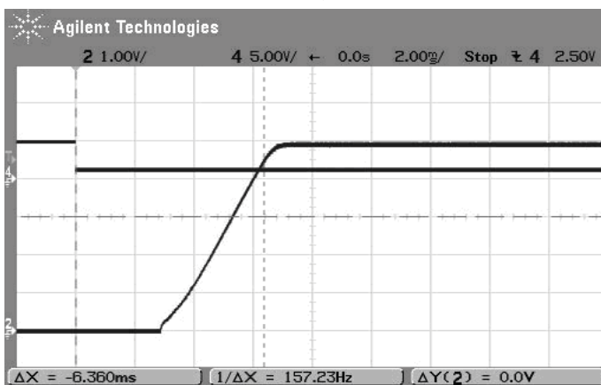
On/Off Enable Startup Delay (Vin=12V, Vout=5V, Iout=3A, Clod=0) Trace 4=Enable In, Trace2=Vout
