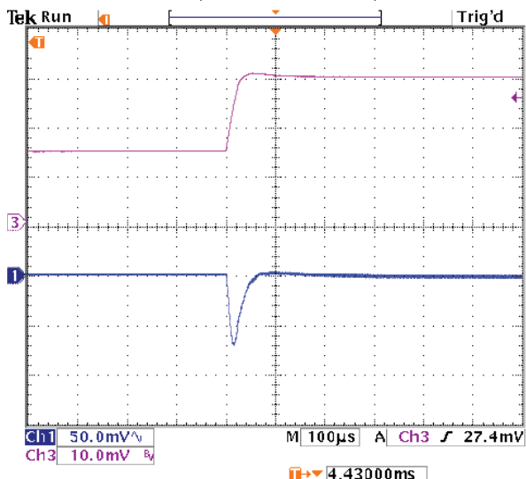
Step Load Transient Response (Vin=12V, Vout=2.5V, Cload=0, Iout=1.5A to 3A) Trace 1=Vout, 50 mV/div. Trace 3=Iout, 1A/div.
