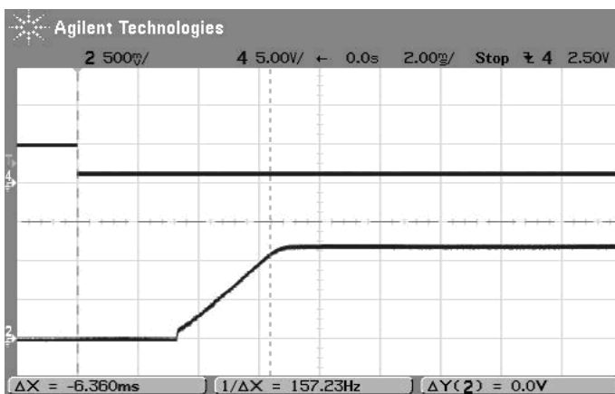
On/Off Enable Startup Delay (Vin=12V, Vout=1.2V, Iout=3A, Clad=0) Trace 4=Enable In, Trace2=Vout
