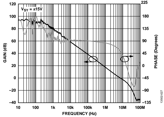
Figure 26. Open-Loop Gain and Phase vs. Frequency, V_{SY} = \pm 15\text{ V}
