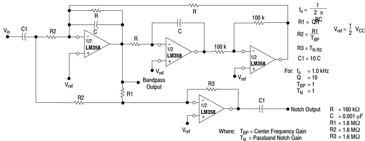
Figure 14. Bi-Quad Filter
