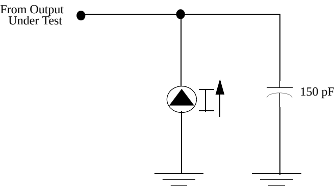
Figure 7. Test Load Diagram
