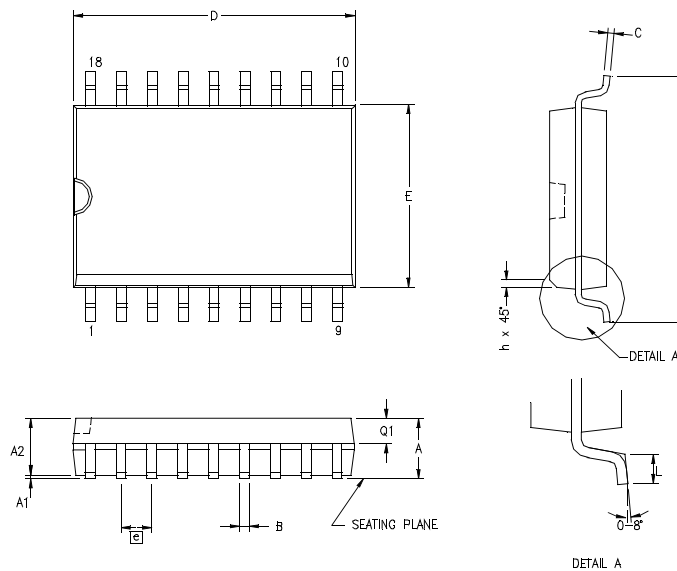
Figure 21. 18-Pin SOIC Package Diagram
