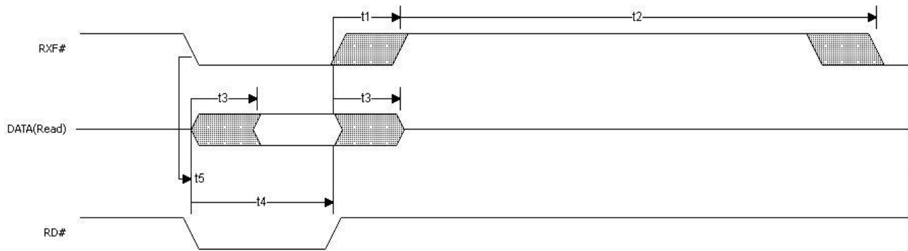
Write Timing
