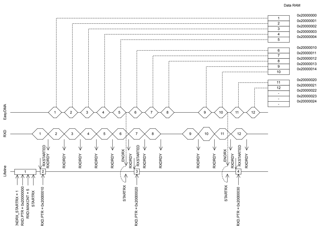
Figure 149: UARTE reception
