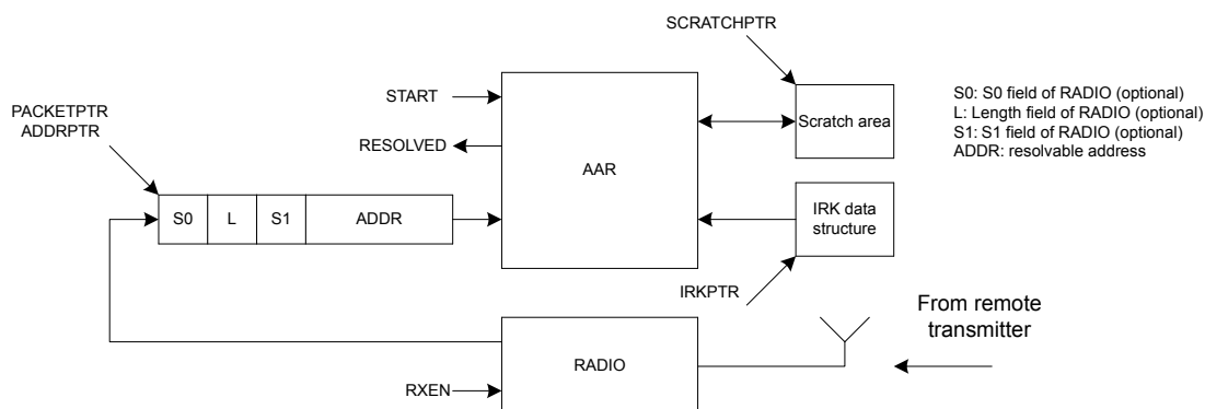
Figure 24: Address resolution with packet loaded into RAM by the RADIO
