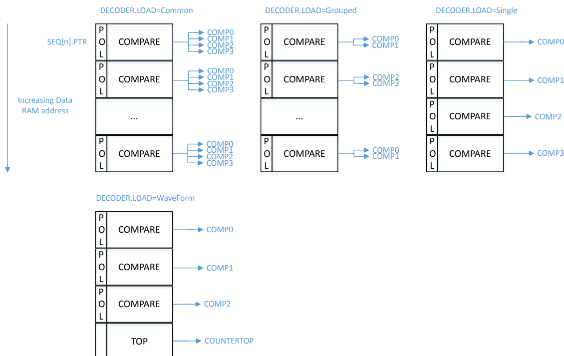
Figure 50: Decoder memory access modes
