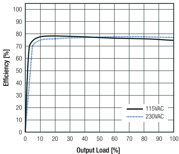
RAC05-3.3SK
