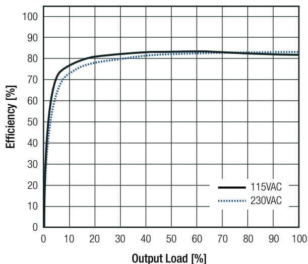
RAC05-12SK
