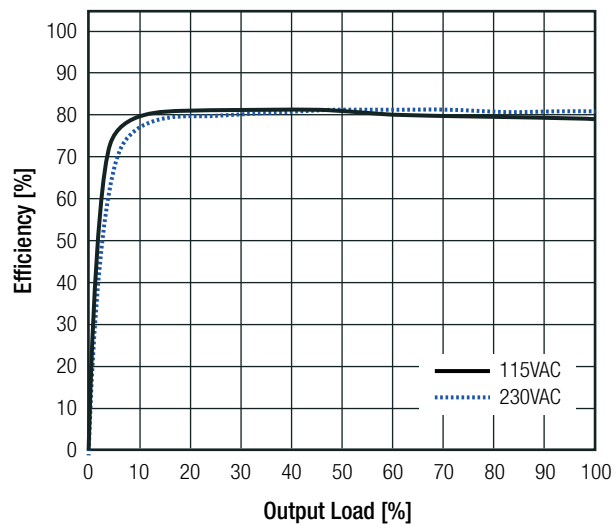
RAC05-05SK
