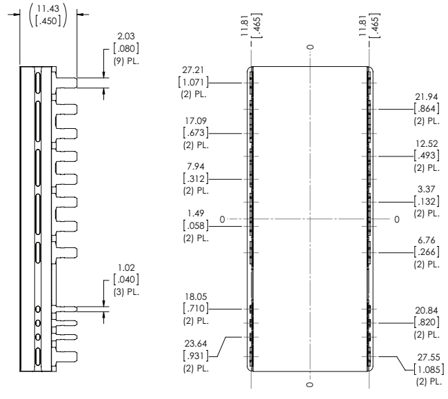
BOTTOM VIEW
