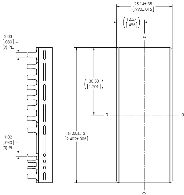
TOP VIEW (COMPONENT SIDE)
