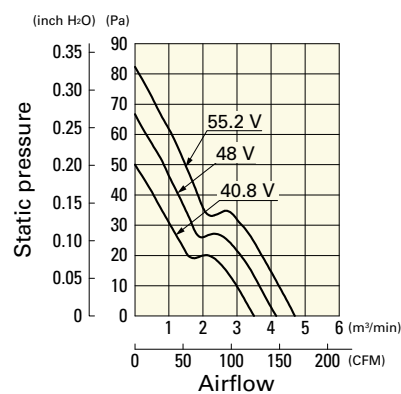
109E5748M501 With pulse sensor
