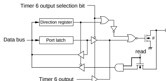
(6) Port P44
