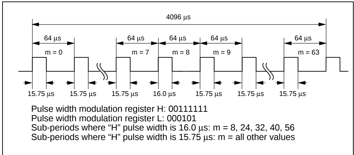
Fig. 57 PWM timing
