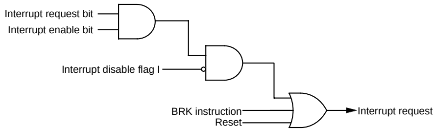
Fig. 15 Interrupt control
