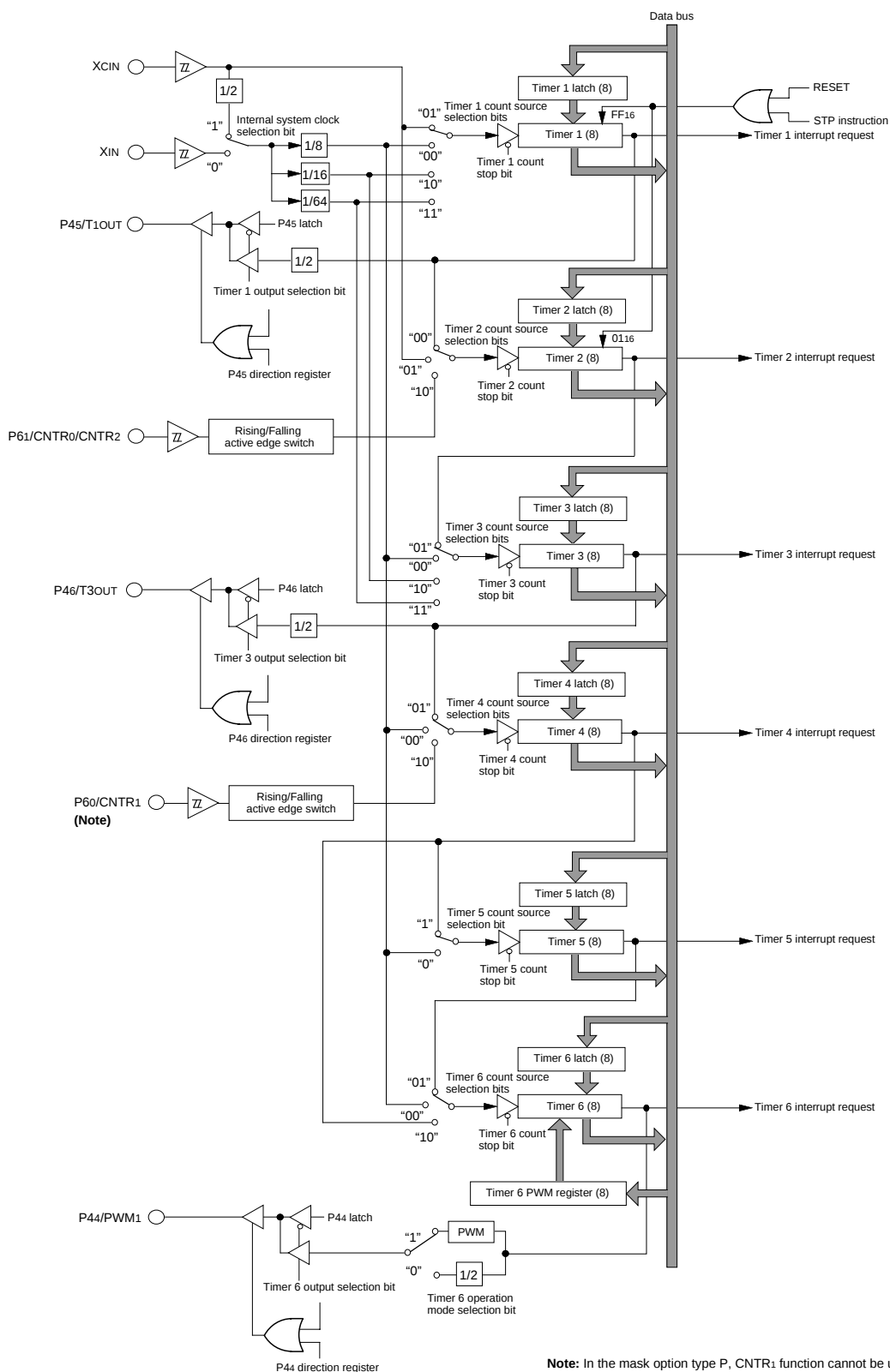
Fig. 18 Block diagram of timer
