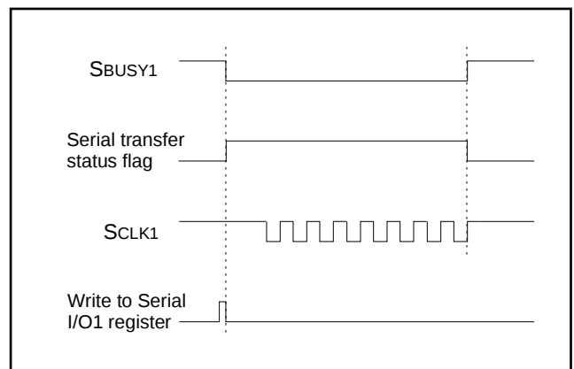
Fig. 31 S BUSY1 output operation (external synchronous clock, 8-bits serial I/O)
