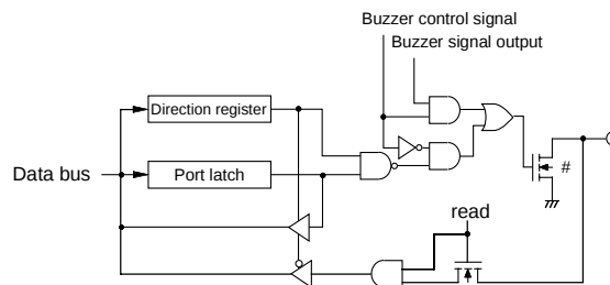
(4) Port P43
