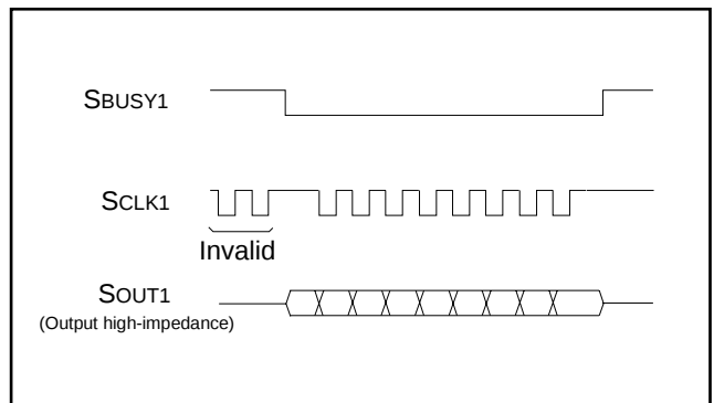
Fig. 29 S BSY1 input operation (external synchronous clock)
