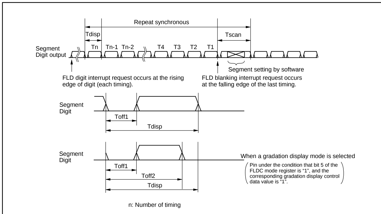
Fig. 51 FLDC timing
