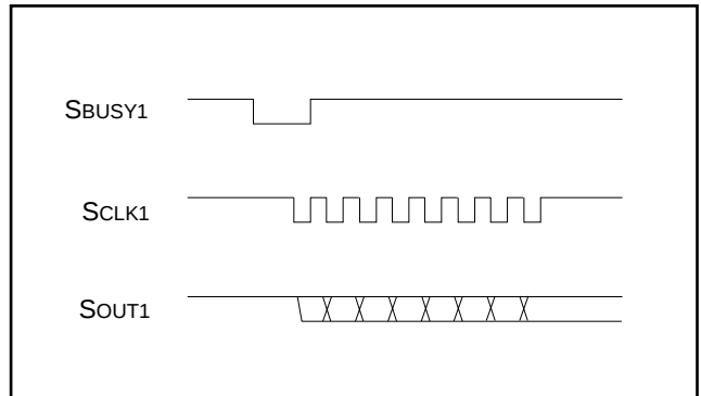
Fig. 28 S BSY1 input operation (internal synchronous clock)
