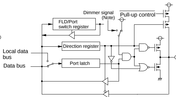
(18) Port P84
