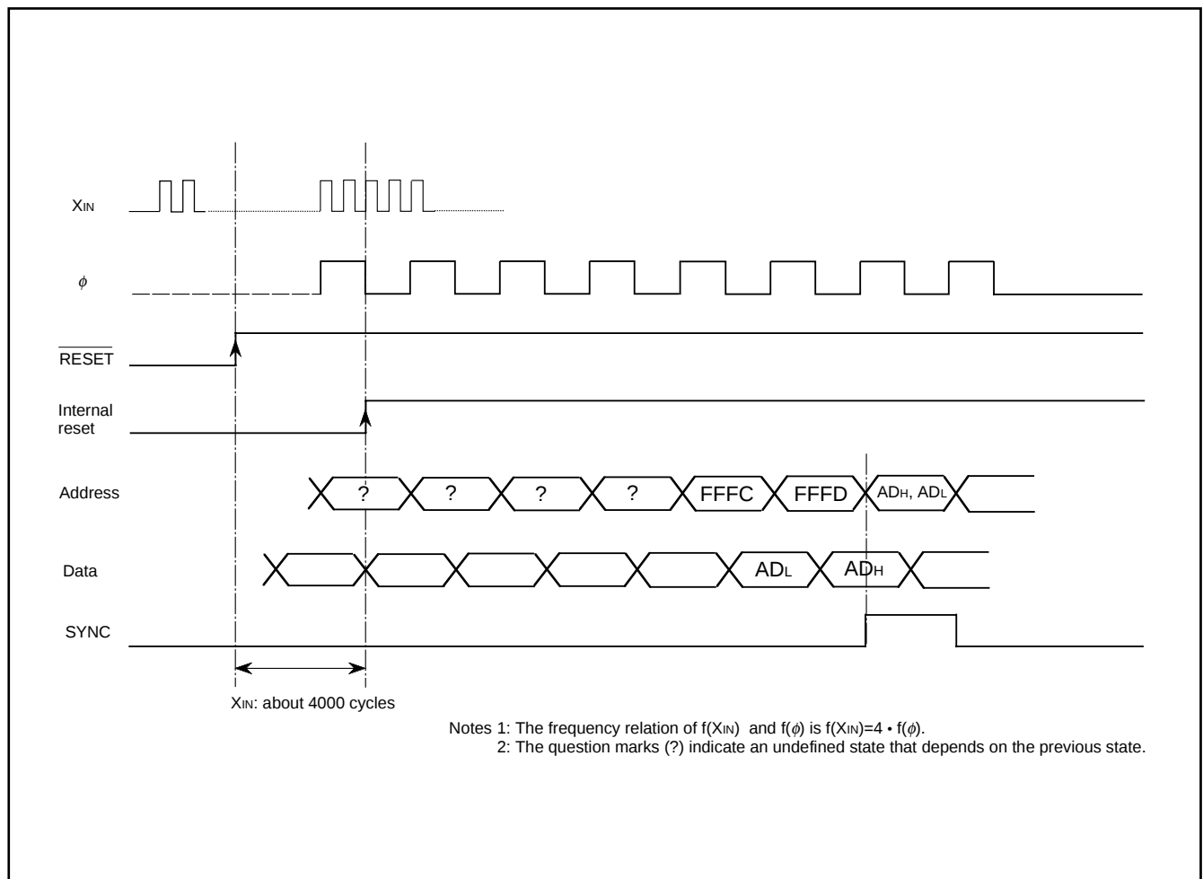
Fig. 69 Reset sequence
