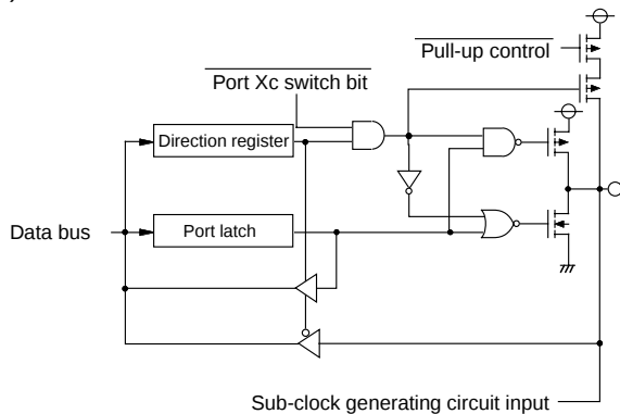
(21) Port P90
