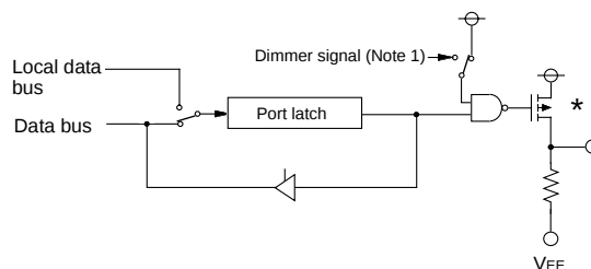
(4) Port P43
