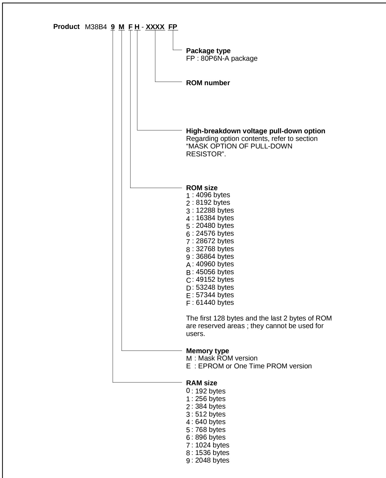
Fig. 3 Part numbering
