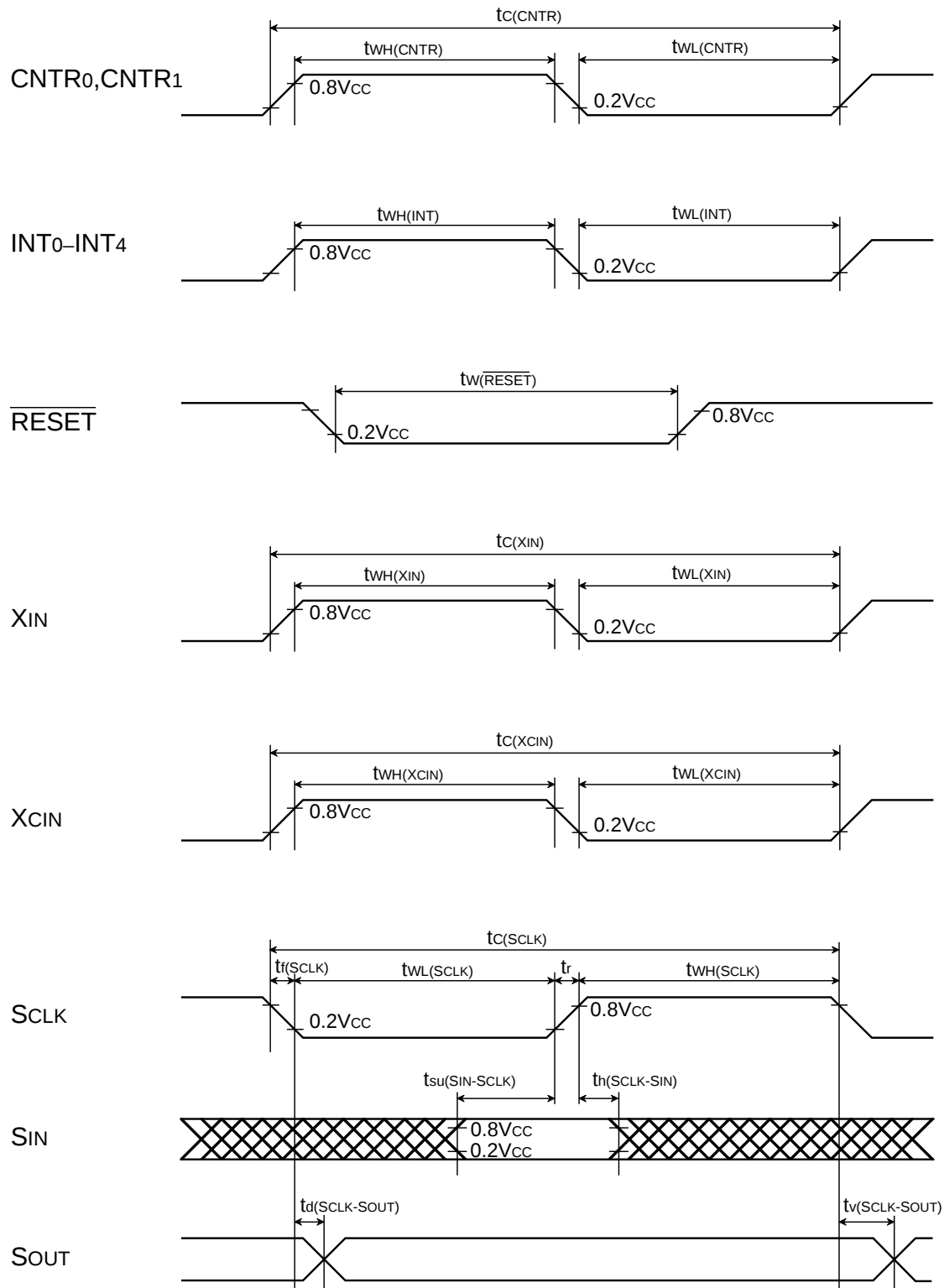
Fig. 78 Timing diagram
