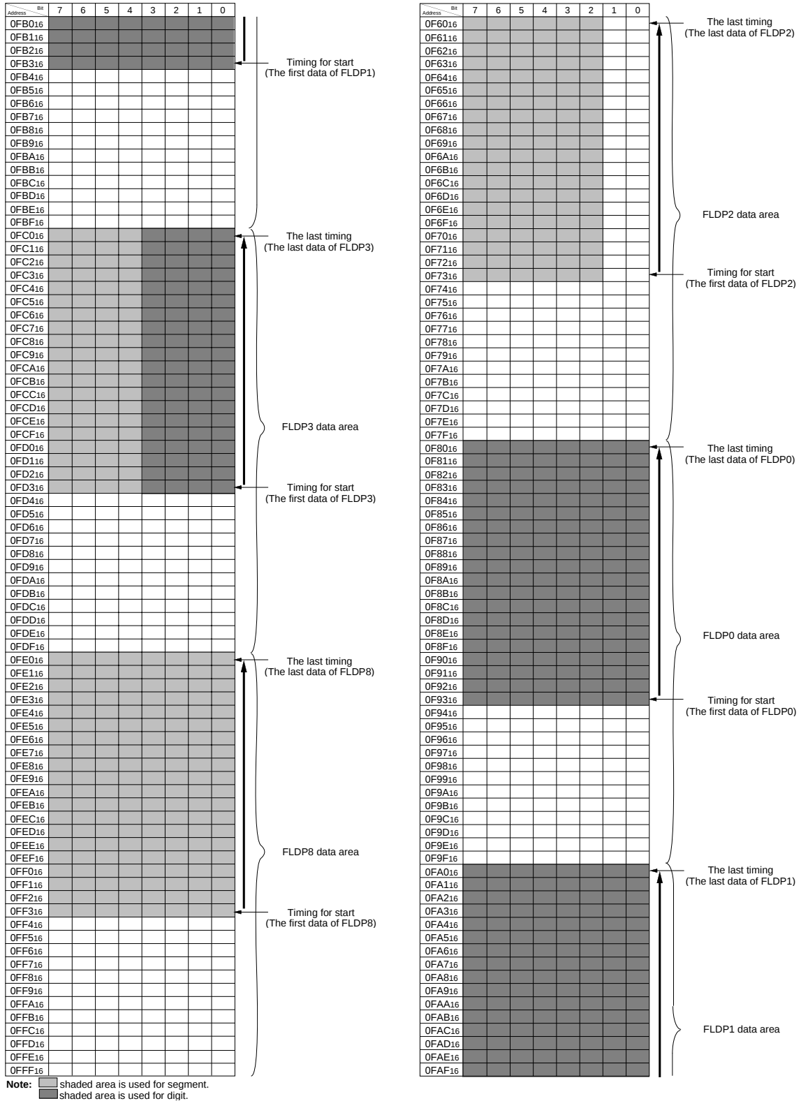
Fig. 48 Example of using FLD automatic display RAM in 32-timing mode
