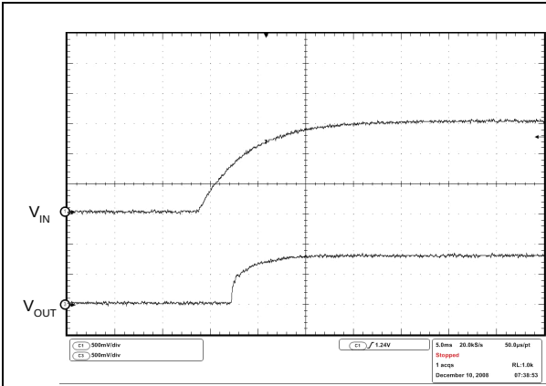
Figure 16. Start-up transient
