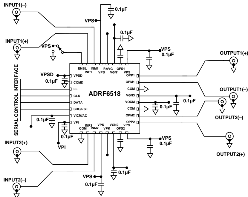
Figure 72. Basic Connections
