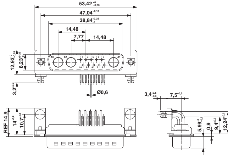
Dimensioned drawing
