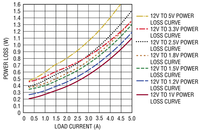
Figure 10. 12V Input Power Loss (Ch1 and Ch2)
