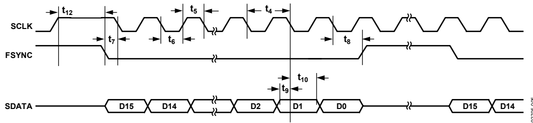
Figure 5. Serial Timing
