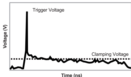
Generalized PulseGuard Suppressor Response to ESD (Positive and Negative Polarity ESD Pulses)
