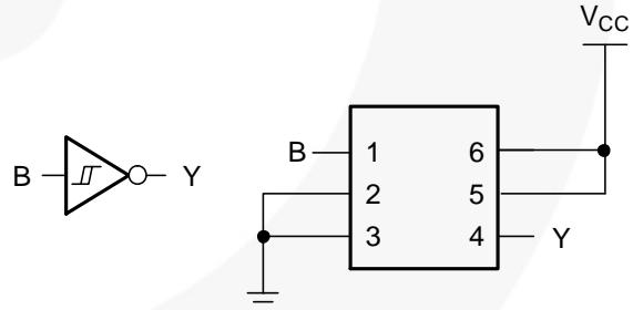
Figure 7. Inverter
