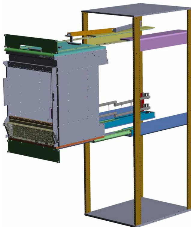
Mounting to support complete extraction from a rack for rear access and maintenance
