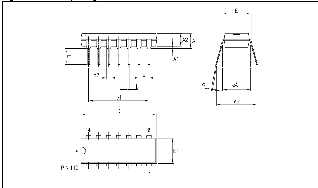
Figure 15. DIP14 package outline
