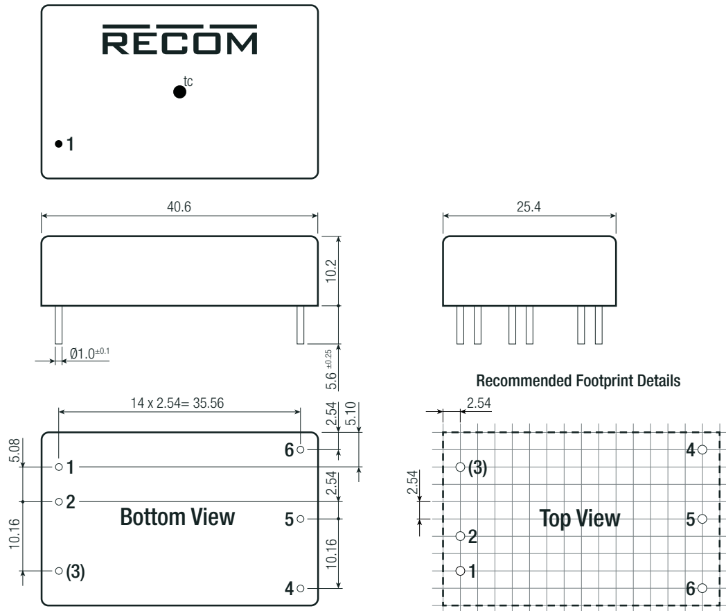
Dimension Drawing (mm)
