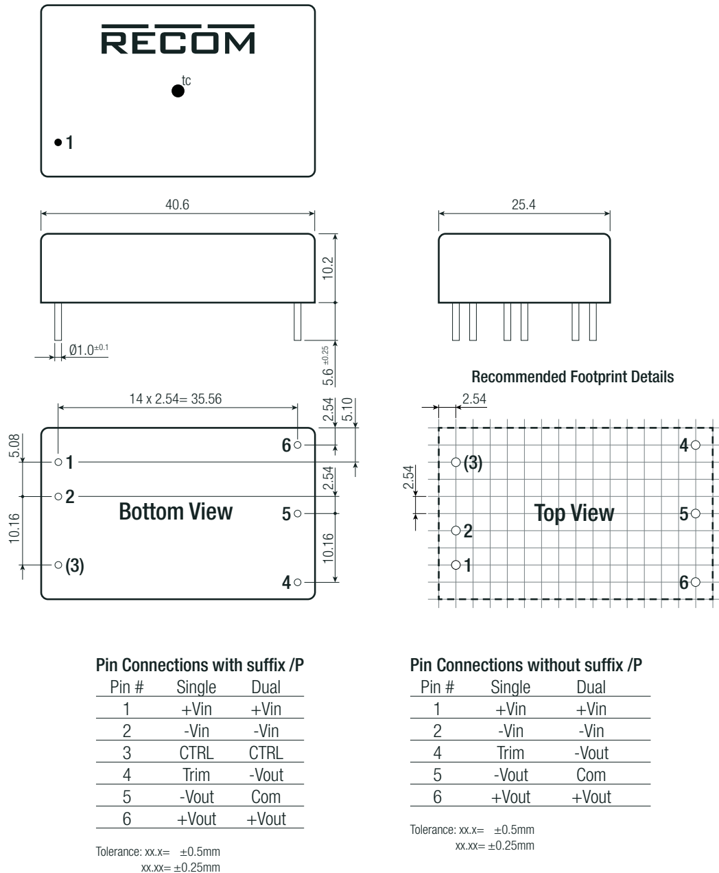
Dimension Drawing (mm)
