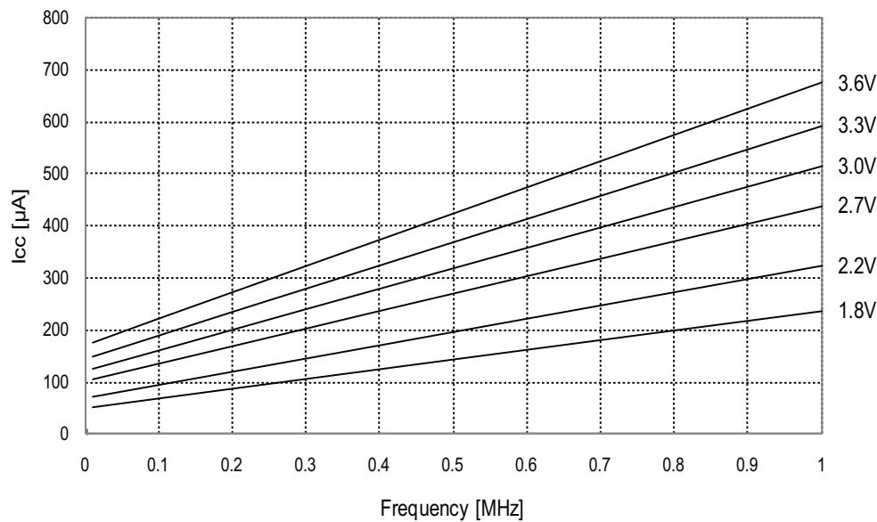
Figure 33-143. Active Supply Current vs. Frequency f_{SYS} = 0 - 1\text{MHz} external clock, T = 25^{\circ}\text{C}
