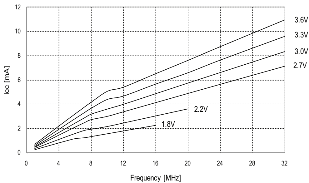
Figure 33-144. Active Supply Current vs. Frequency f_{SYS} = 1 - 32\text{MHz} external clock, T = 25^{\circ}\text{C}
