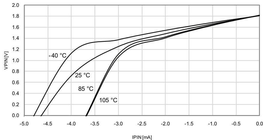
Figure 33-163. I/O Pin Output Voltage vs. Source Current V_{CC} = 1.8V
