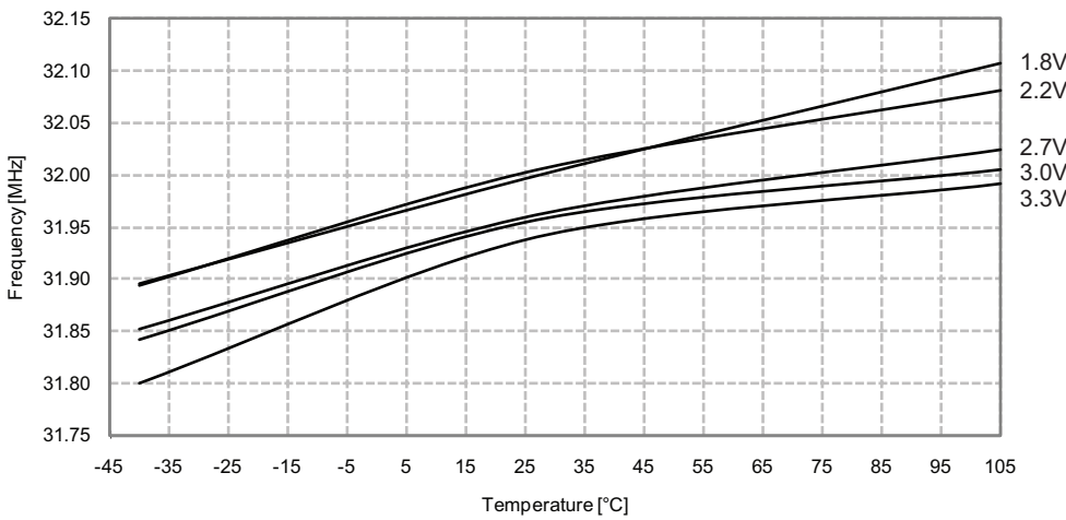
Figure 33-342. 32MHz Internal Oscillator Frequency vs. Temperature DFLL enabled, from the 32.768kHz internal oscillator
