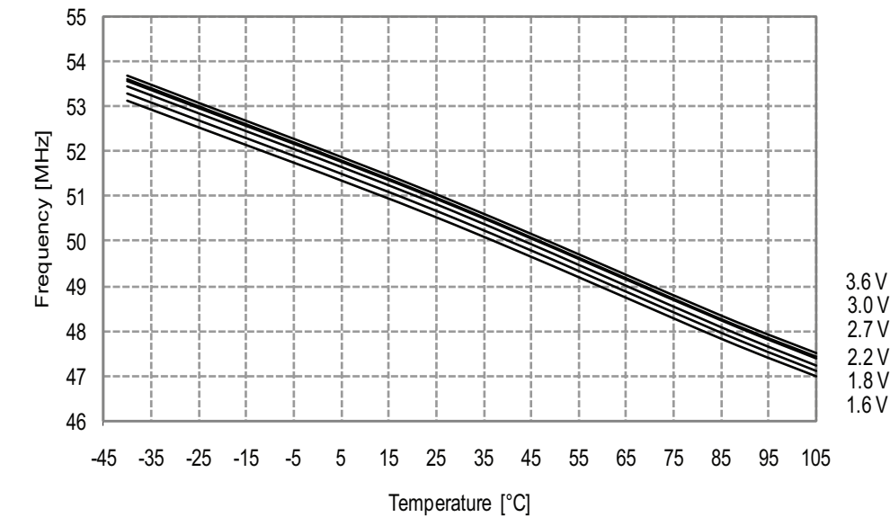
Figure 33-68. 48MHz Internal Oscillator Frequency vs. Temperature DFLL enabled, from the 32.768kHz internal oscillator
