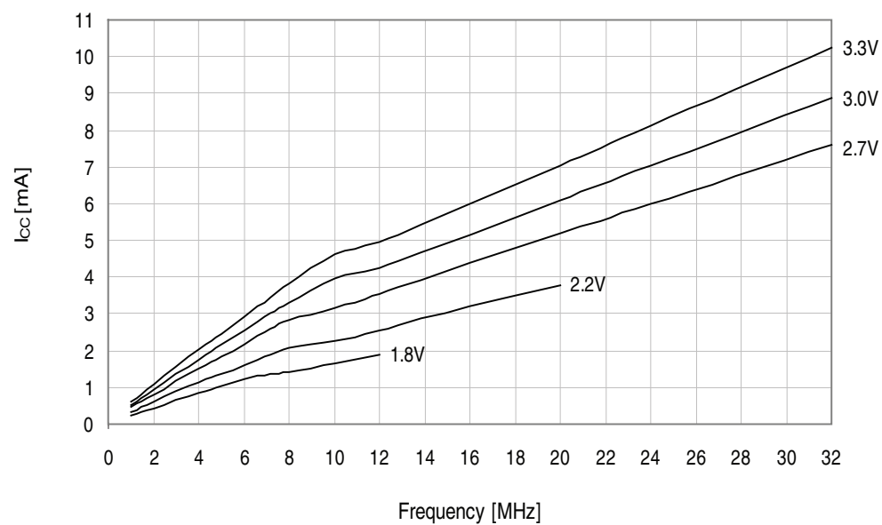
Figure 33-214.Active Supply Current vs. Frequency f_{SYS} = 1 - 32\text{MHz} external clock, T = 25^{\circ}\text{C}
