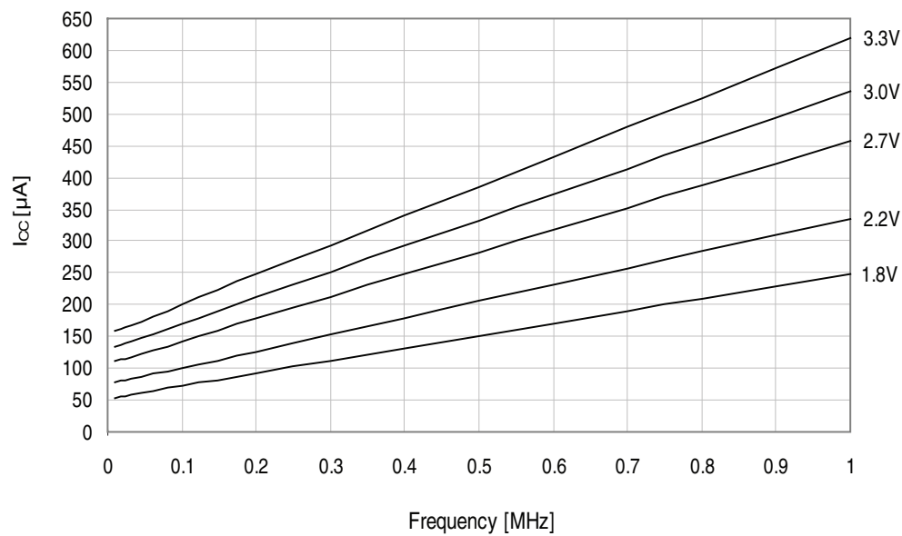
Figure 33-213.Active Supply Current vs. Frequency f_{SYS} = 0 - 1\text{MHz} external clock, T = 25^{\circ}\text{C}
