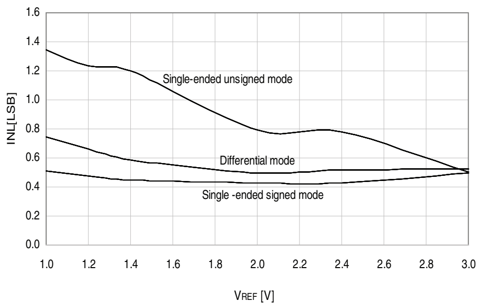
Figure 33-312. INL Error vs. External V_{REF} T = 25^{\circ}\text{C} , V_{CC} = 3.6\text{V} , external reference
