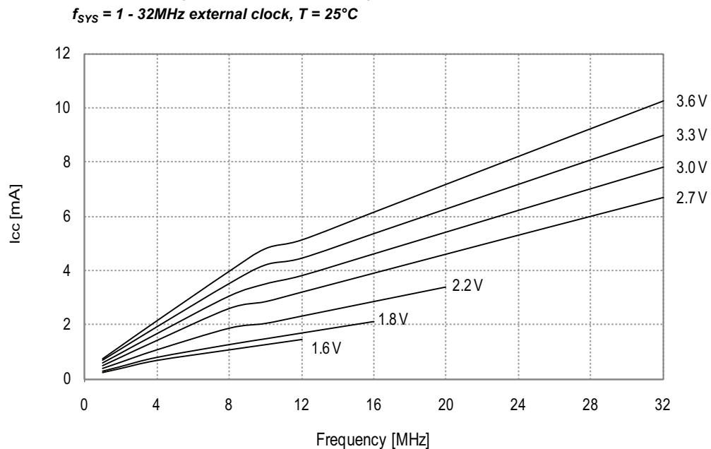
Figure 33-73. Active Supply Current vs. Frequency
