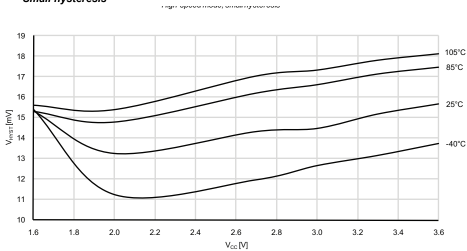
Figure 33-323. Analog Comparator Hysteresis vs. V_{CC} Small hysteresis
