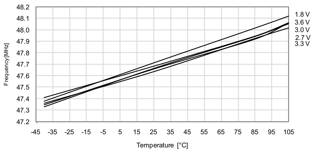
Figure 33-209. 48MHz Internal Oscillator Frequency vs. Temperature DFLL enabled, from the 32.768kHz internal oscillator
