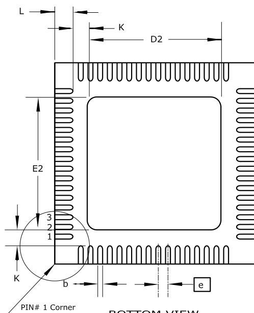
BOTTOM VIEW
