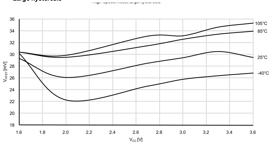
Figure 33-324. Analog Comparator Hysteresis vs. V_{CC} Large hysteresis
