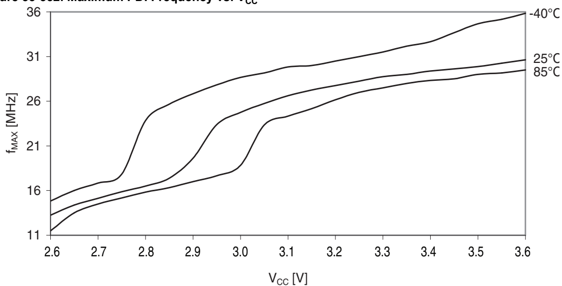
Figure 33-352. Maximum PDI Frequency vs. V_{CC}
