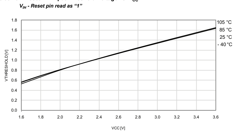
Figure 33-194. Reset Pin Input Threshold Voltage vs. V_{CC}
