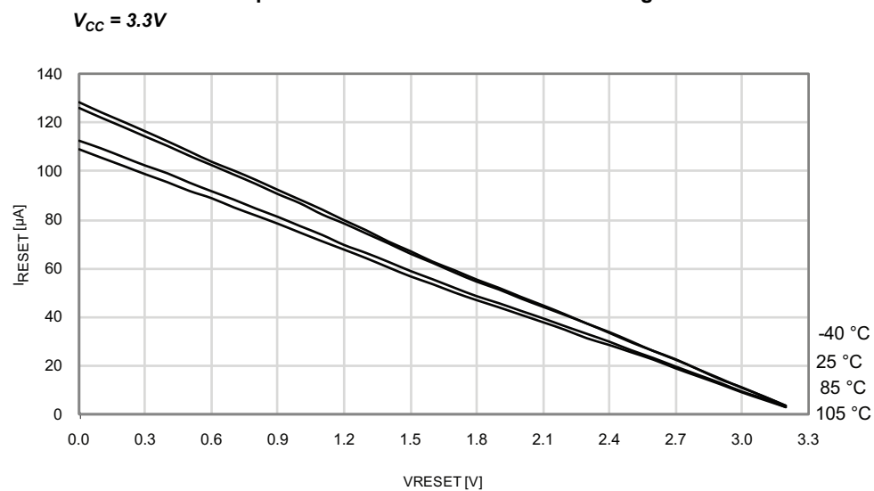
Figure 33-193. Reset Pin Pull-up Resistor Current vs. Reset Pin Voltage
