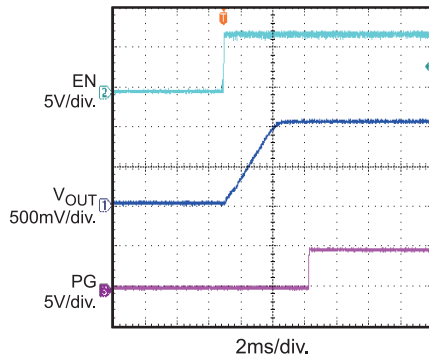
Power Good Through EN Start-Up C_{SS} = 33nF
