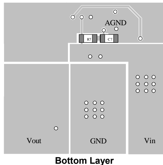
Figure 15—PCB Layout
