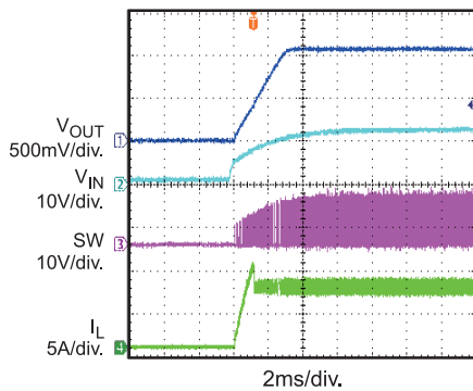
Start-Up Through VIN I_{OUT} = 7A
