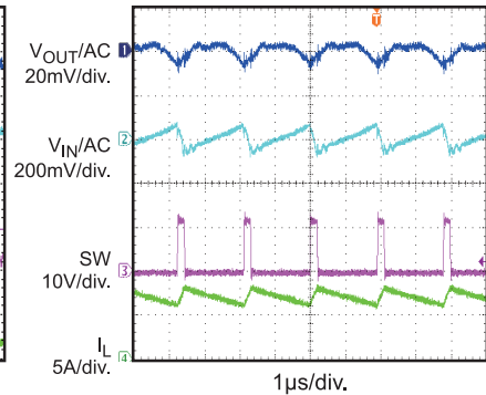
Input/Output Voltage Ripple I_{OUT} = 7A
