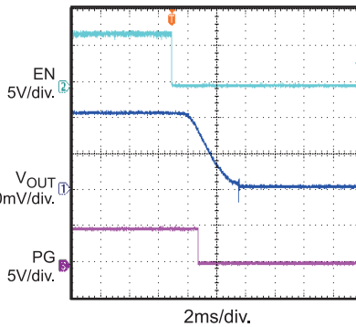
Power Good Through EN Shutdown C_{SS} = 33nF
